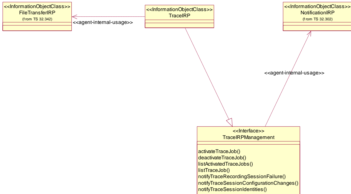
Figure 6.1: Class Diagram
