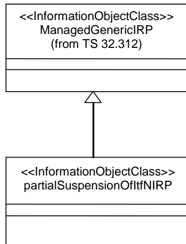
Figure 5.2.2-1: Inheritance Diagram
