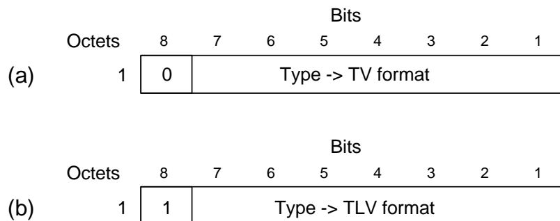
Figure 6.2: Type field for (a) TV and (b) TLV format
