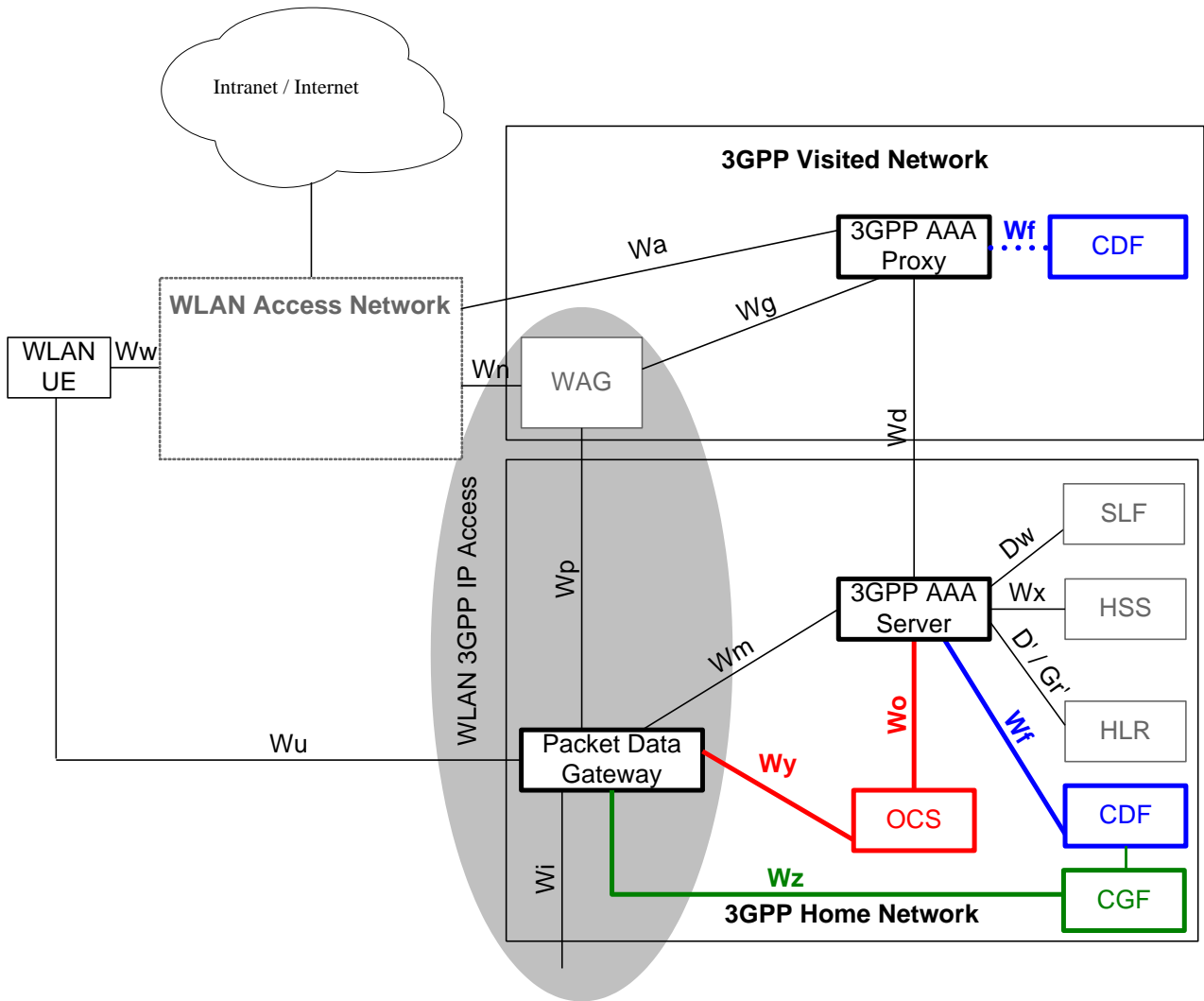
Figure 4.1.3: Roaming reference model - 3GPP PS based services provided via the 3GPP Home Network
