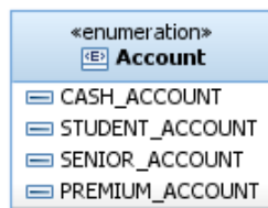
Figure 18: <<enumeration>> notation
