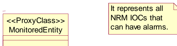
<<ProxyClass>> Notation
