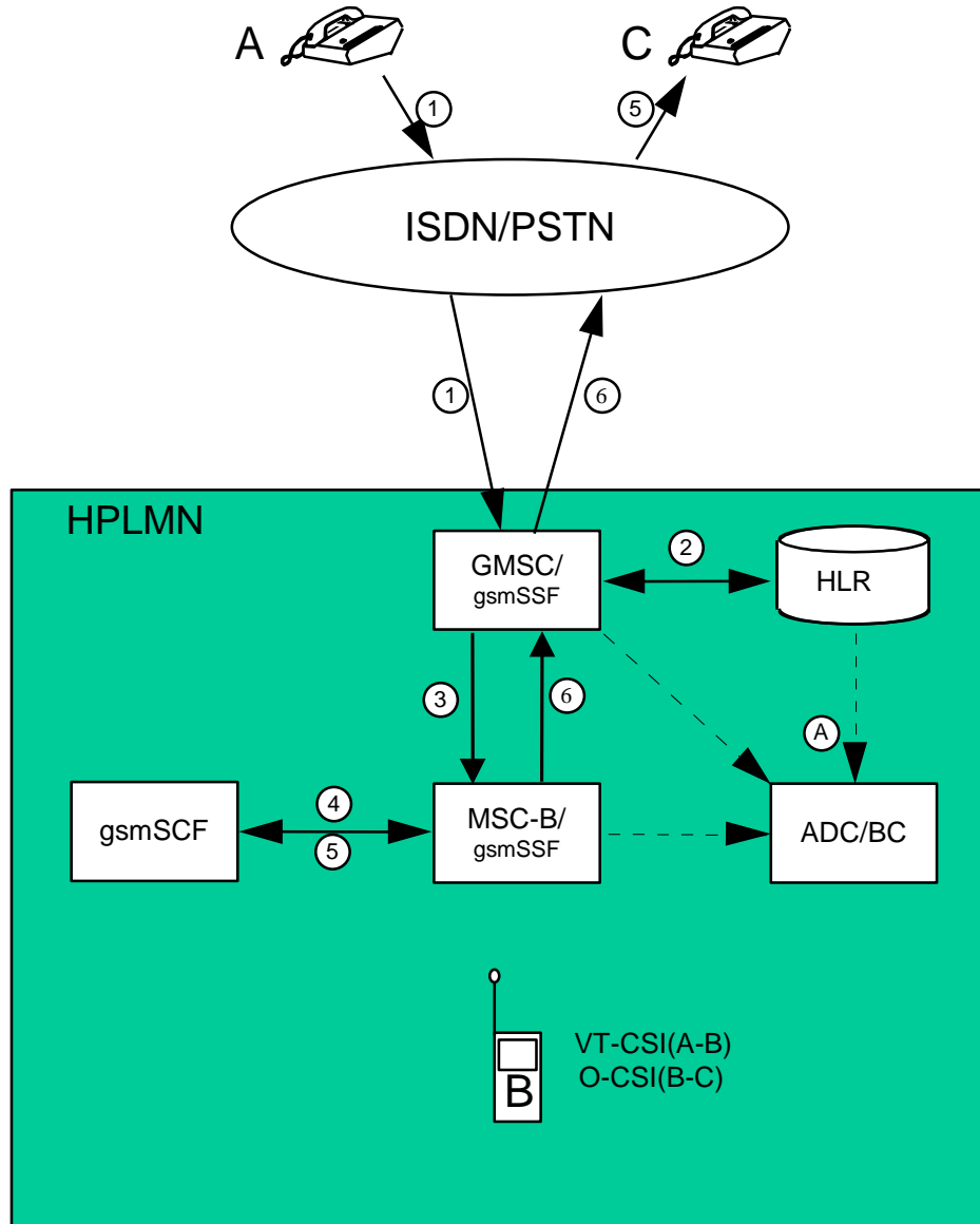
Figure B.20: Incoming call handled by CAMEL with redirection decided and forwarding leg handled by CAMEL in VMSC
