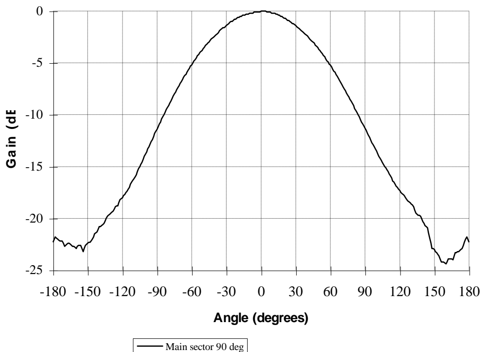
Figure 1.5.1: Horizontal antenna pattern
