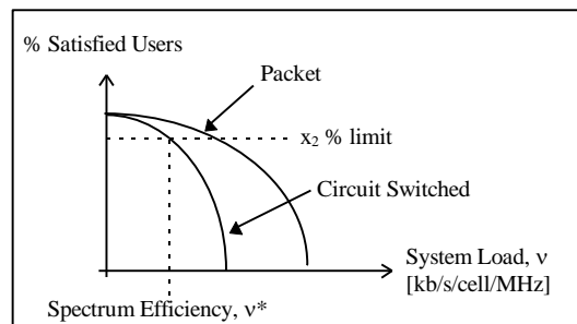
Figure 1.6.A: Example of spectrum efficiency for a mixed service scenario with one circuit switched service and one packet service.
