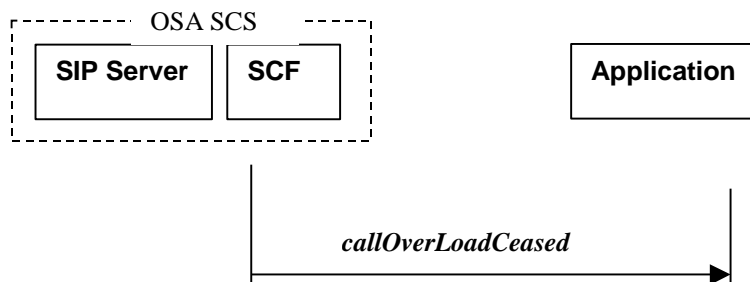
Figure 5-13: Call flow for callOverLoadCeased()
