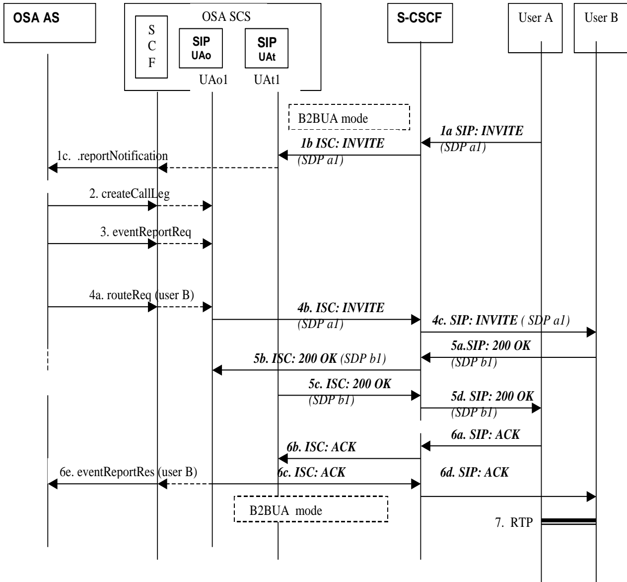
Figure B-3: Example user Initiating OSA SCS Flow for Two Party call Set-up
