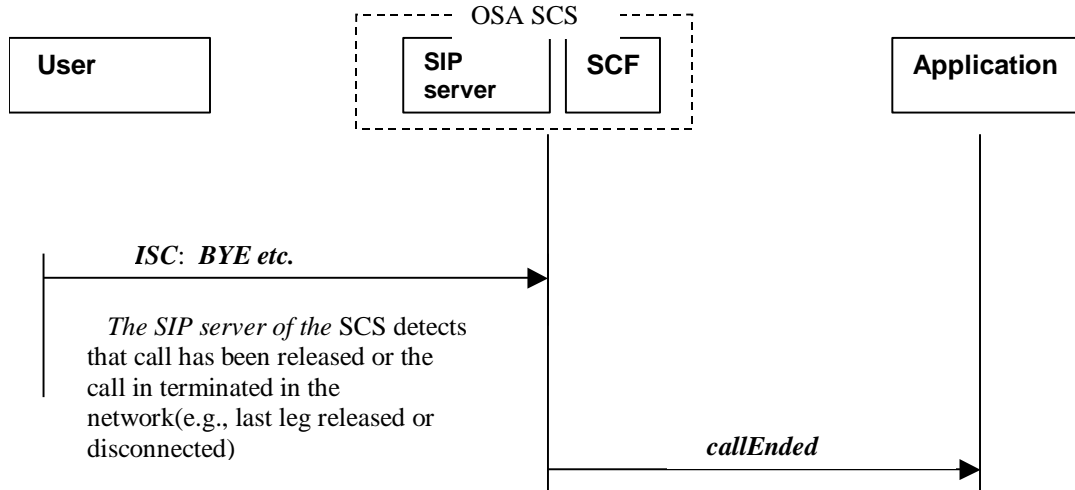
Figure 5-25: Call flow for callEnded()
