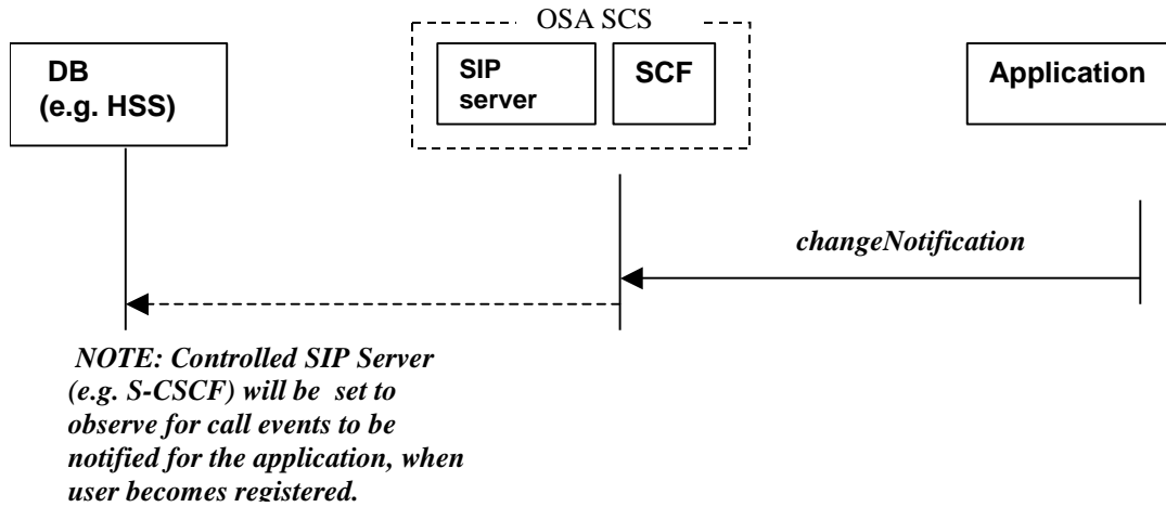
Figure 5-3: Call flow for changeNotification()
