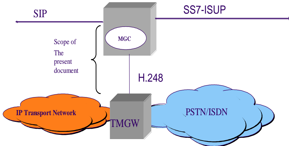
Figure 1: Reference architecture
