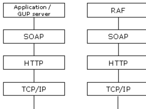
Figure 7.2.2 GUP Rp reference point protocol architecture
