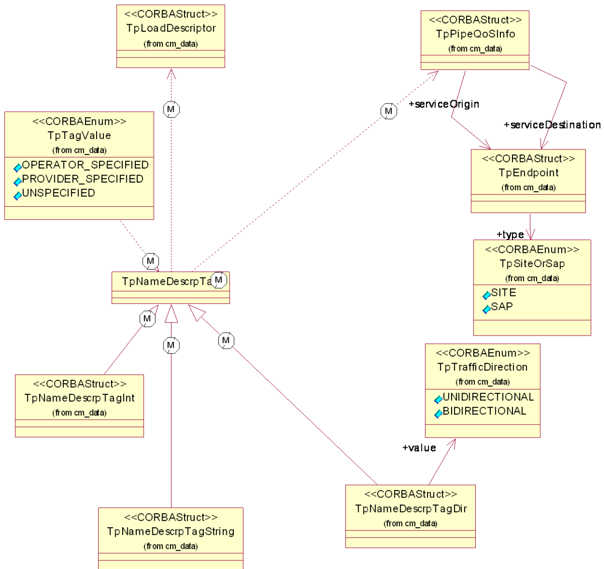
Figure : Pipe QoS Data Types
