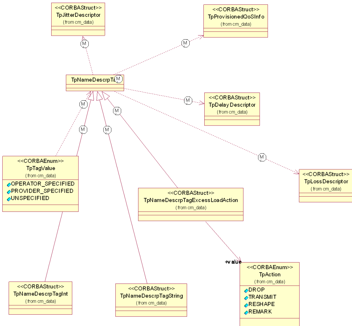
Figure : Provisioned QoS Data Type Classes
