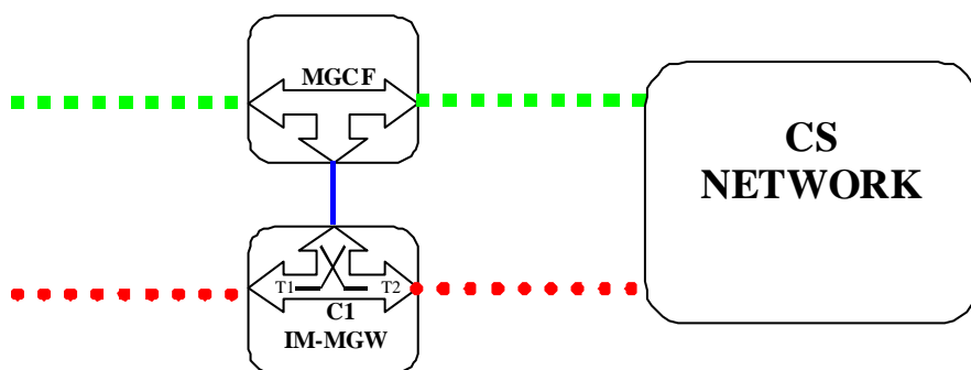
Figure 33: Network model
