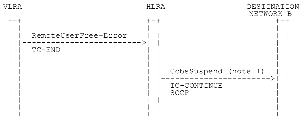
Figure 6.4: Signalling flow for CCBS Suspend Invocation (RemoteUserFree_Result)
