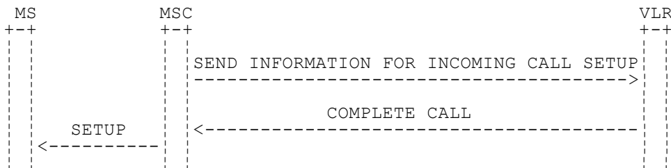
Figure 5.1: Signalling for CLIP supplementary service
