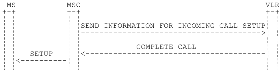
Figure 5.4: Signalling for COLR supplementary service
