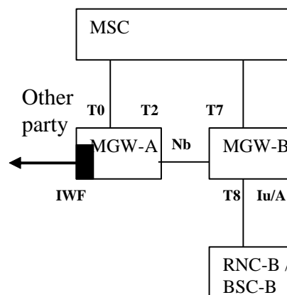
Figure 19: Transport on the access side of the IWF if the same MSC server controls one MGW A hosting the IWF and another MGW B interfacing the radio access network
