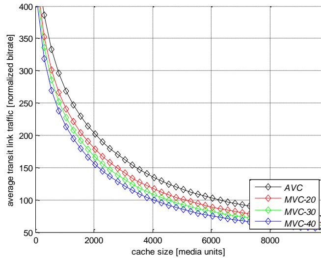
Figure 23: Average traffic through the “transit” link.
