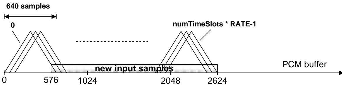
(a) QMF analysis windowing of input signal
