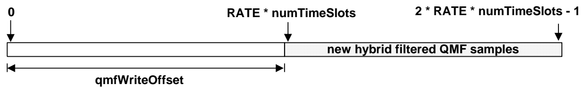
(c) subband sample buffer X
