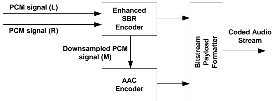
Figure 2 Parametric stereo aacPlus block diagram
