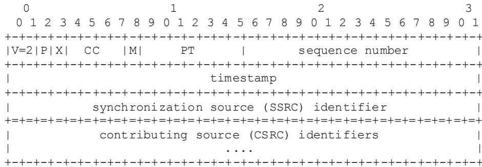
Figure 7-2: RTP HEADER
