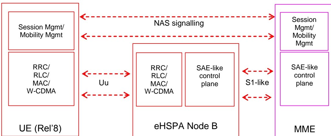
Figure 7.1.5-3: Control plane
