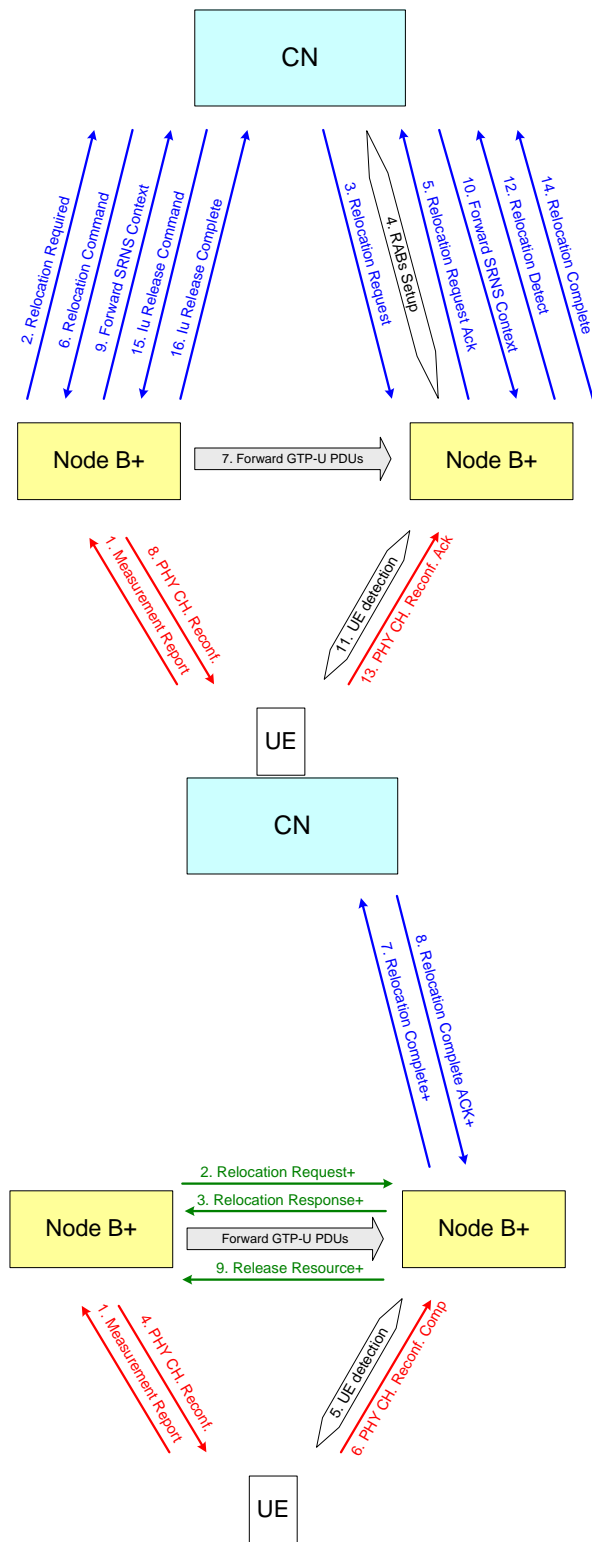
Figure 7.1.7-2: Current vs Enhanced SRNS relocation with hard handover
