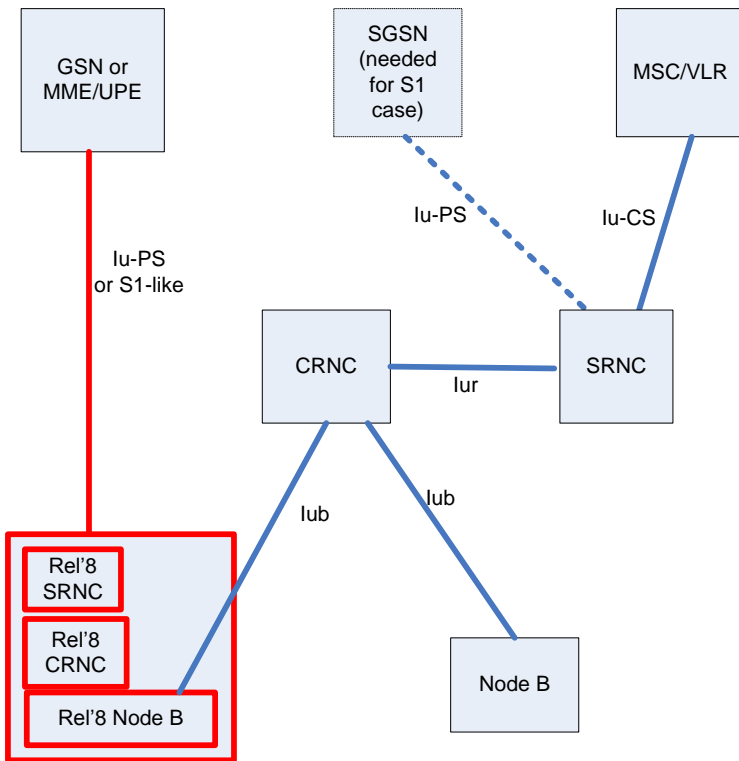
Figure 7.2.3-1: Non-collapsed legacy RNC - eHSPA control plane in the Node B
