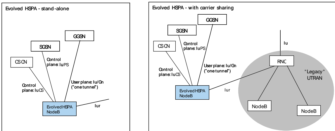
Figure 7.1.4-2: U-Plane & C-Plane functions located in Node-B
