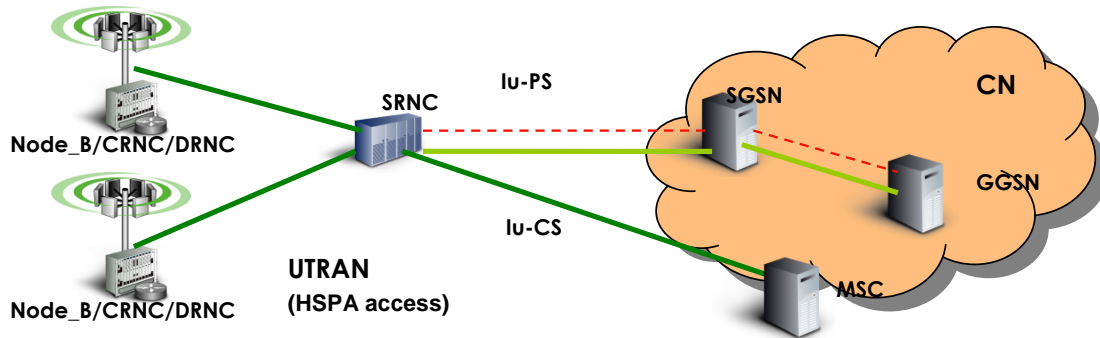
Figure 7.1.2.1-1: Iu with enhanced SRNC separate from the enhanced collapsed CRNC/DRNC/Node B
