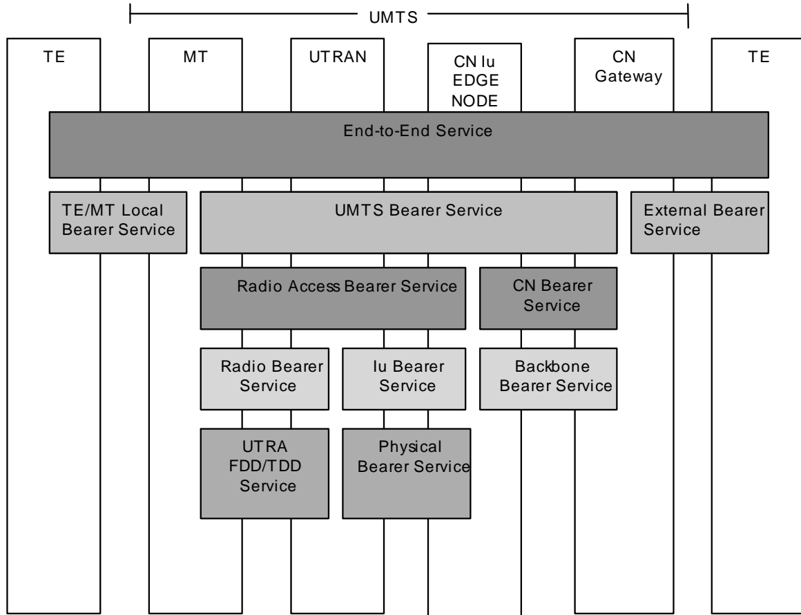
Figure 4.1: UMTS QoS Architecture
