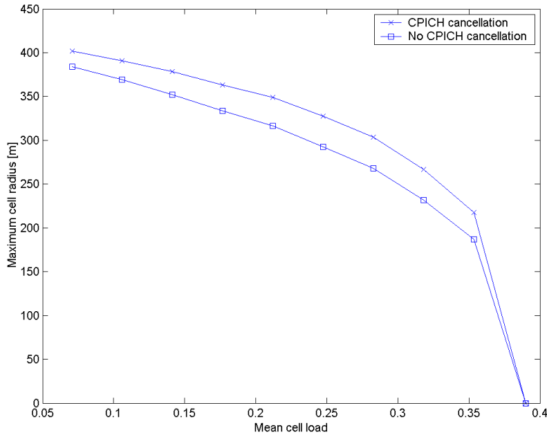
Figure 11: The capacity gain due to CPICH cancellation in an urban environment
