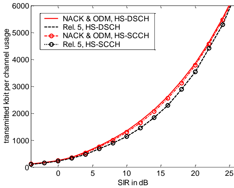
Figure 7: Transmitted amount of data per channel usage
