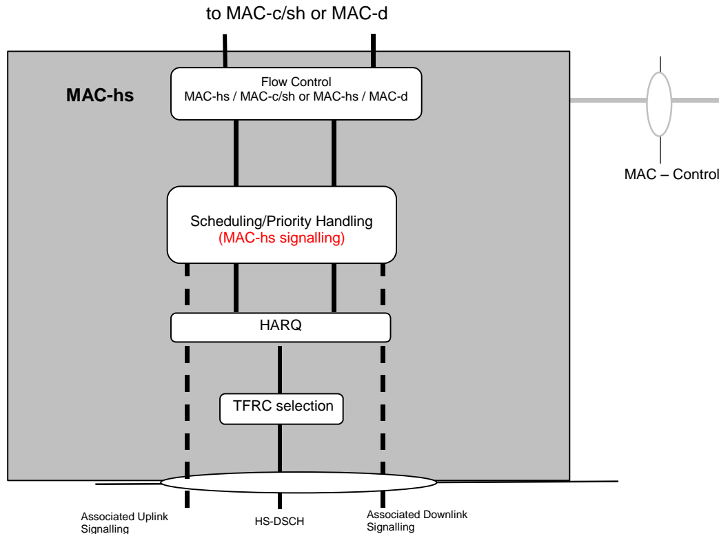
Figure33. MAC-hs function.
