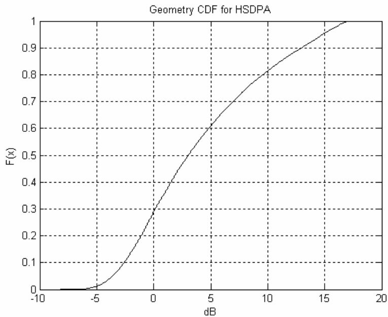
Figure 6.2: Geometry CDF [11]
