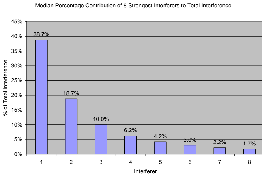
Figure 6.6: 8 Strongest Interferers [10]
