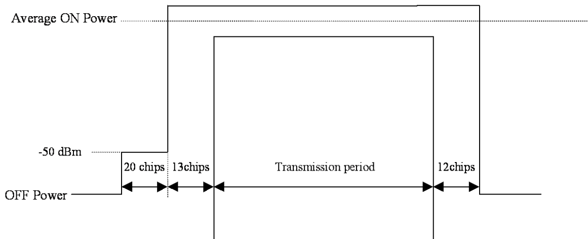
Figure 5.3: Transmit ON/OFF template
