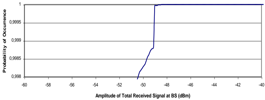
Figure 8.10: CDF of Total Signal for Speech Only System with 5 km Cells and Worst Case Geographic Offset
