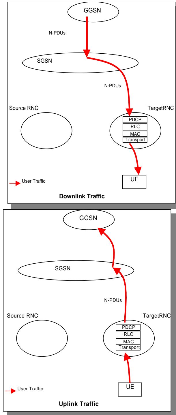
Figure 27: User Plane – Completion phase with only one SGSN
