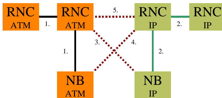
Figure 6-30: Interworking cases
