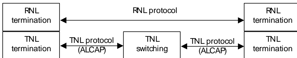
Figure 6-13: RNL and TNL terminations
