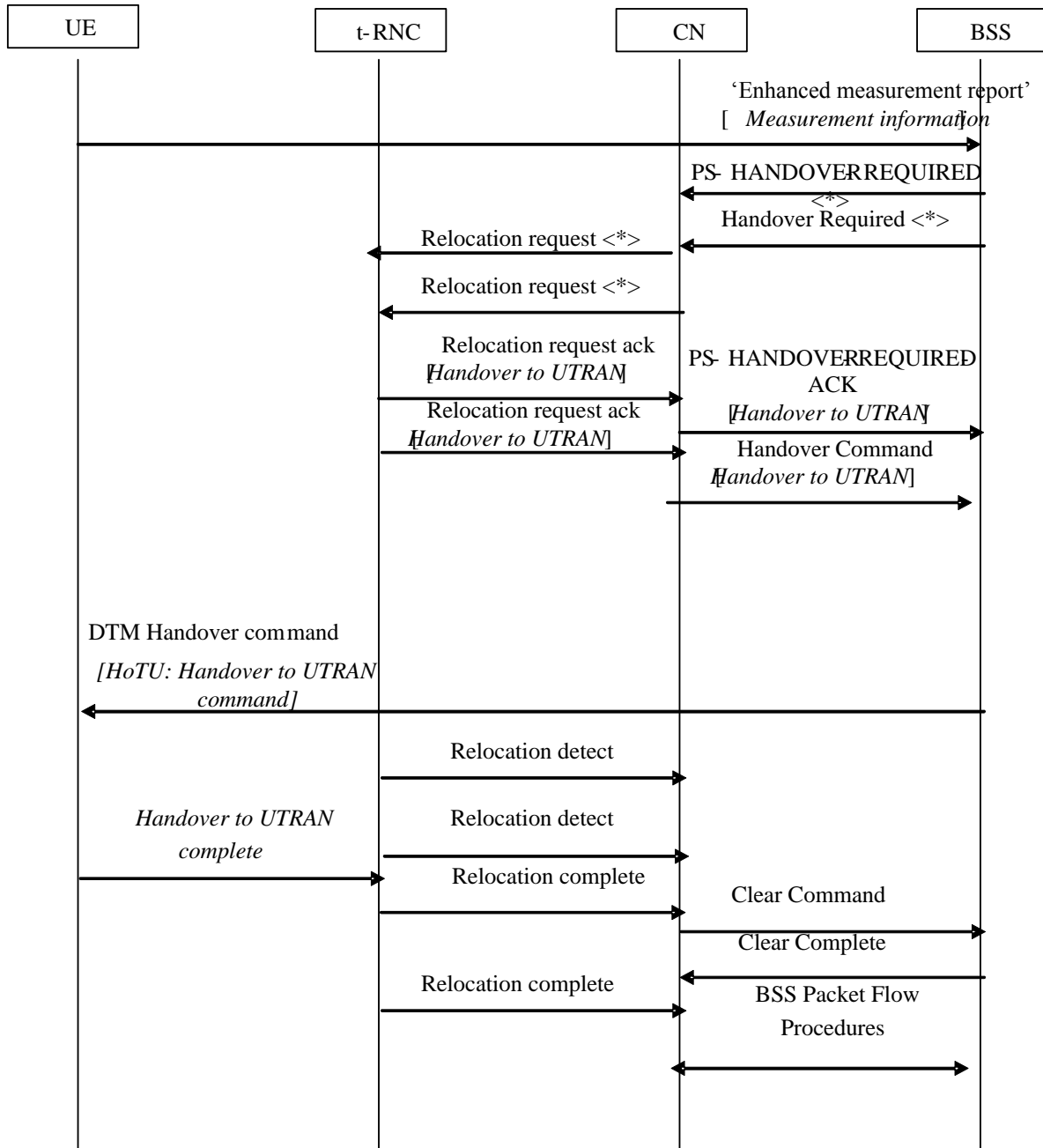
Figure 5.1.5.2.5 – 3 : Inter-RAT DTM Handover to UTRAN from GERAN A/Gb mode
