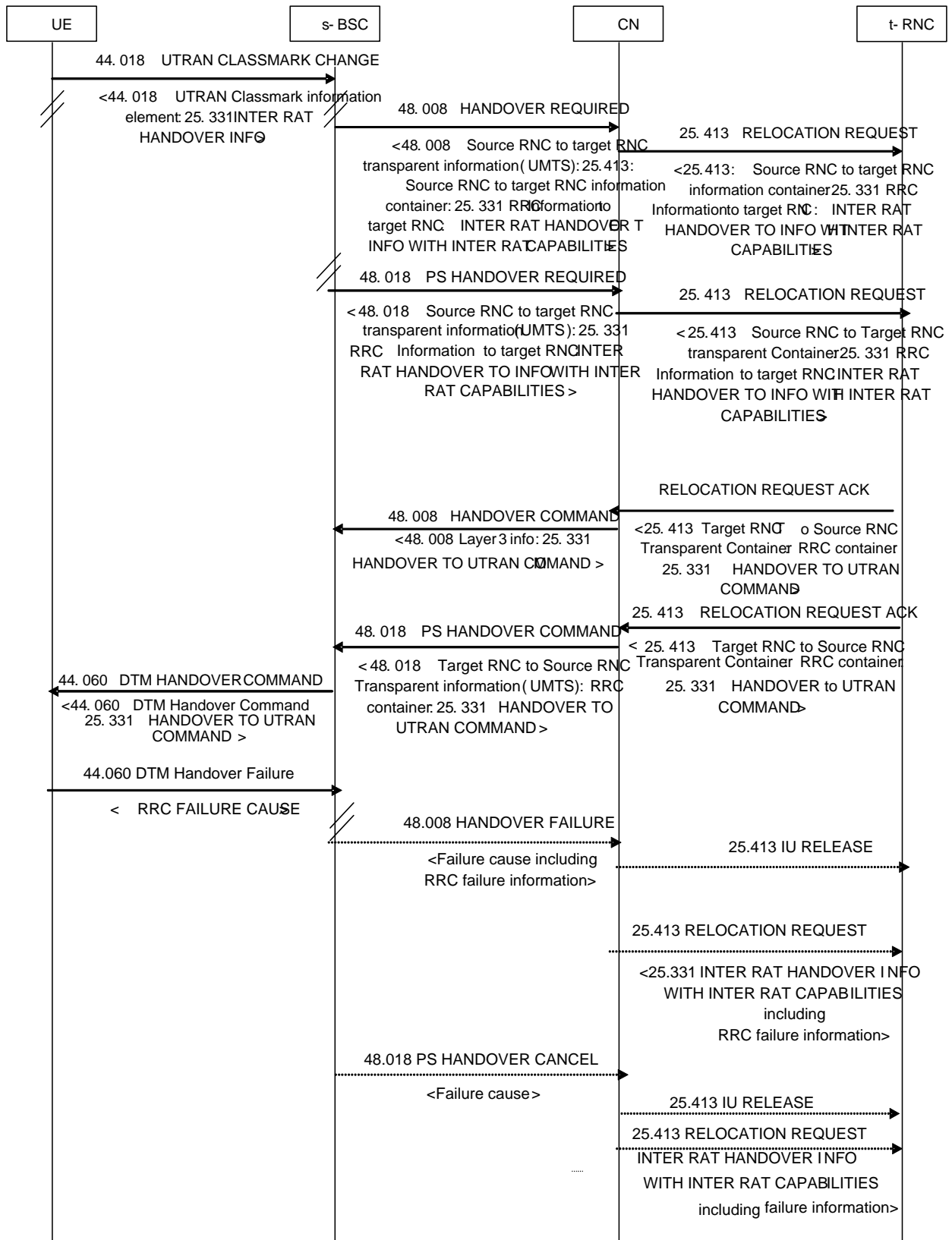
Figure 5.1.7.3-1c: Inter-RAT DTM Handover from GERAN A/Gb mode to UTRAN, failure due to critical extension not supported by UE
