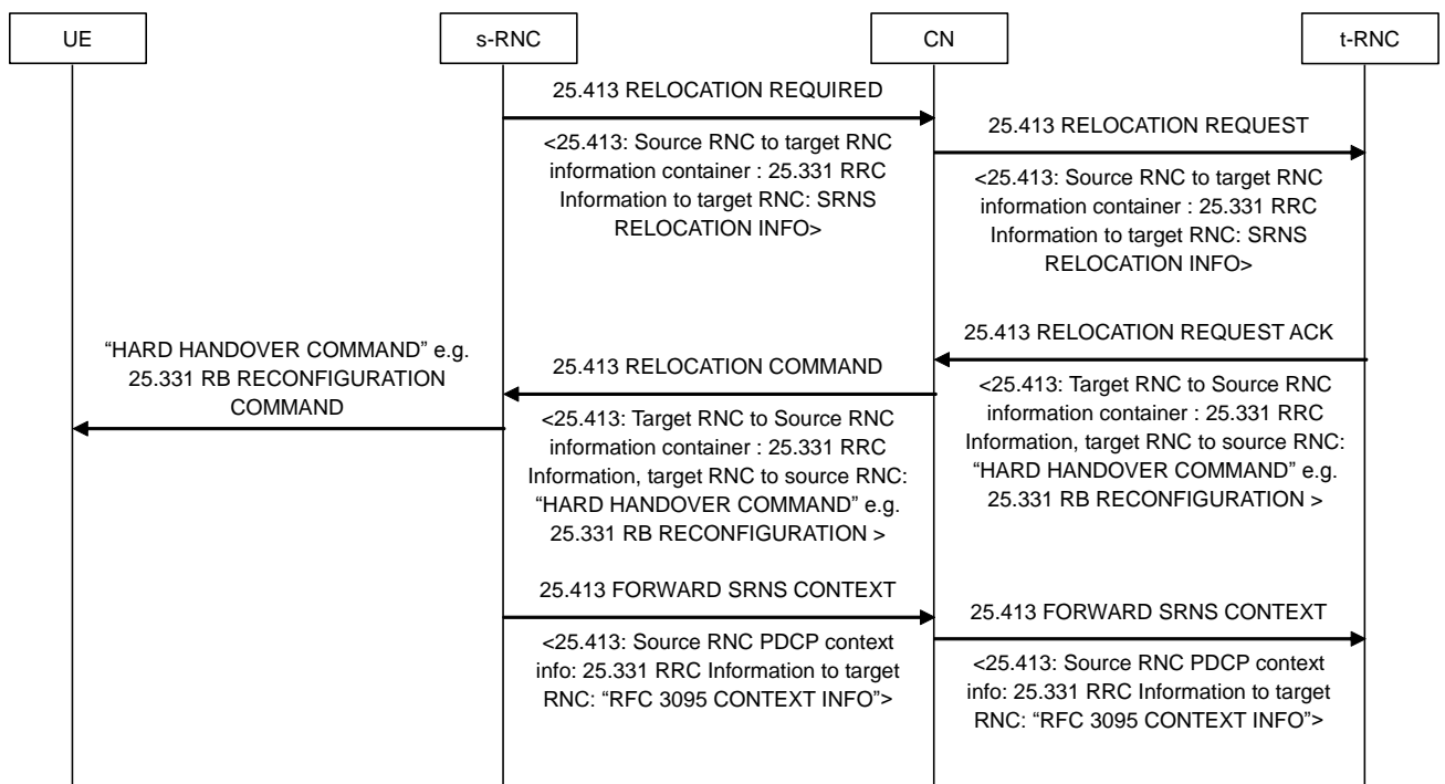
Figure 5.1.7.2-3b: SRNS relocation, flow with context relocation info in FORWARD SRNS CONTEXT
