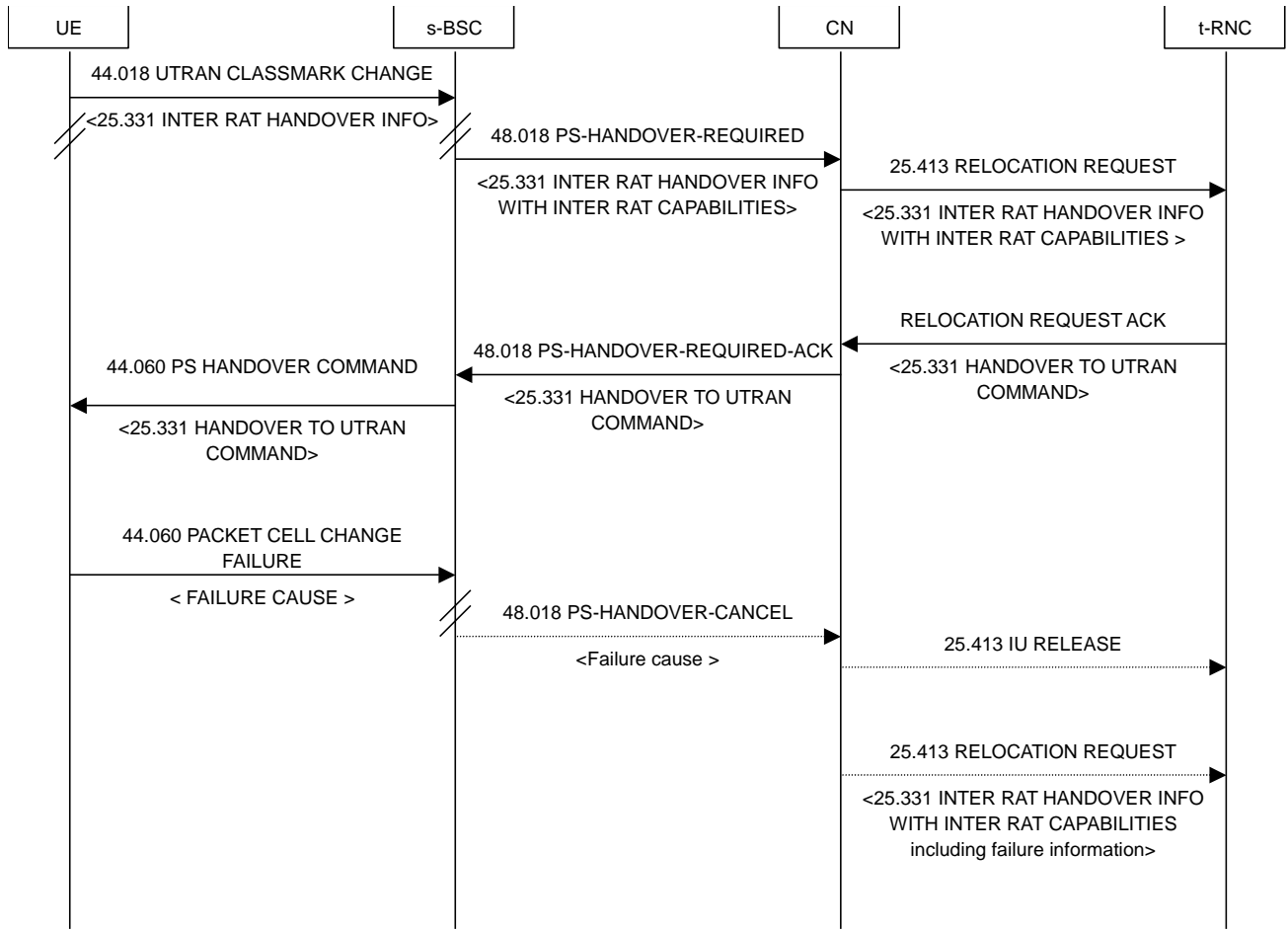
Figure 5.1.7.3-1b: Handover of PS domain service from GERAN A/Gb mode to UTRAN, failure due to critical extension not supported by UE
