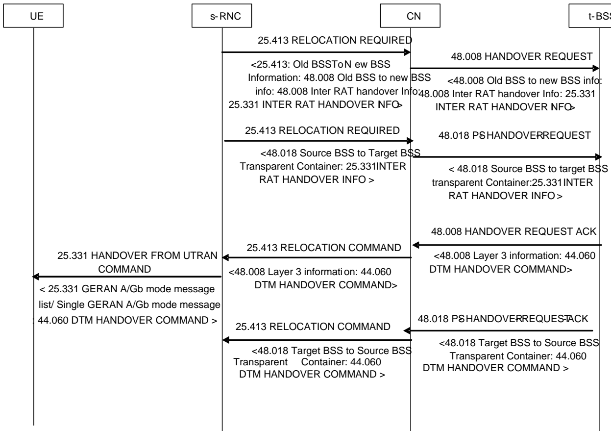
Figure 5.1.7.2-2c. Inter-RAT DTM handover from UTRAN to GERAN A/Gb mode, normal flow
