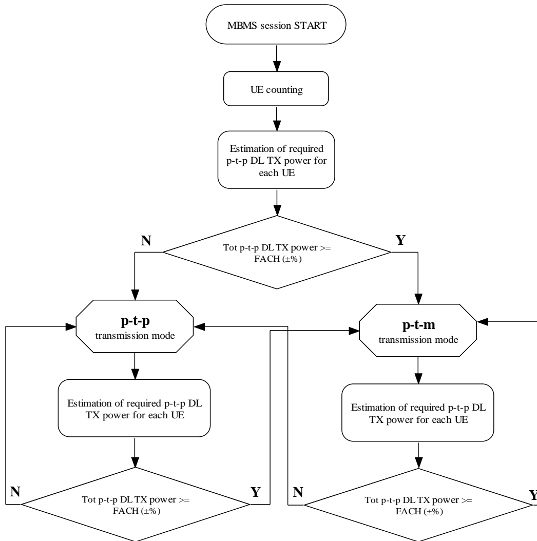
Figure 14.2.3-1: Example of MBMS p-t-p / p-t-m switching algorithm
