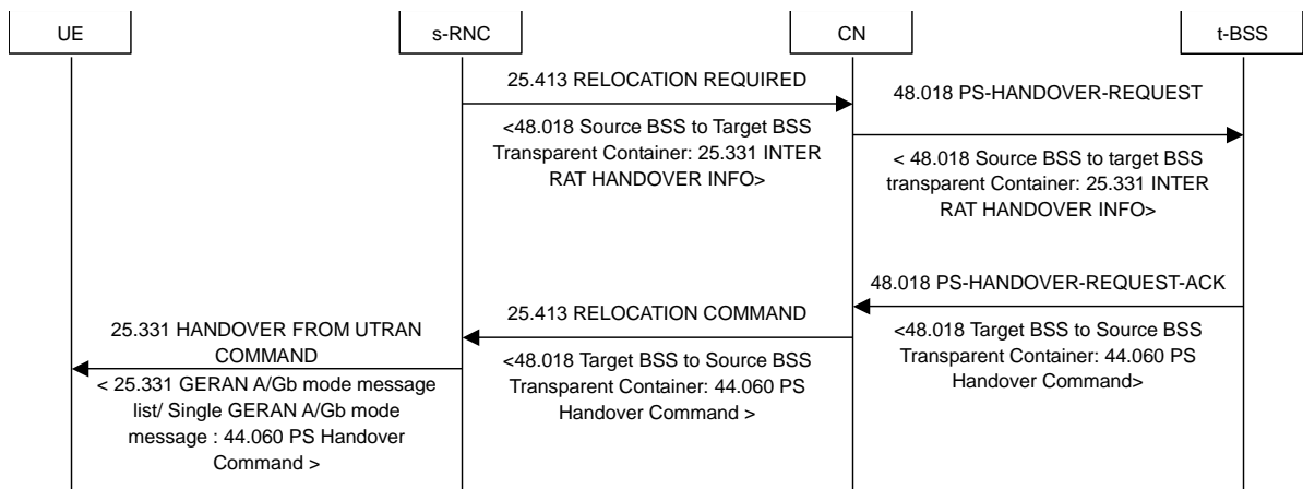
Figure 5.1.7.2-2b. Handover of PS domain service from UTRAN to GERAN A/Gb mode, normal flow
