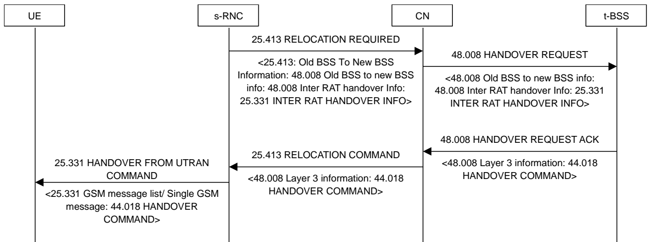
Figure 5.1.7.2-2: Handover of CS domain service from UTRAN to GERAN A/Gb mode, normal flow
