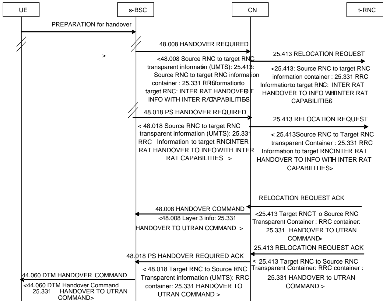
Figure 5.1.7.2-1c. Inter-RAT DTM Handover from GERAN A/Gb mode to UTRAN, normal flow
