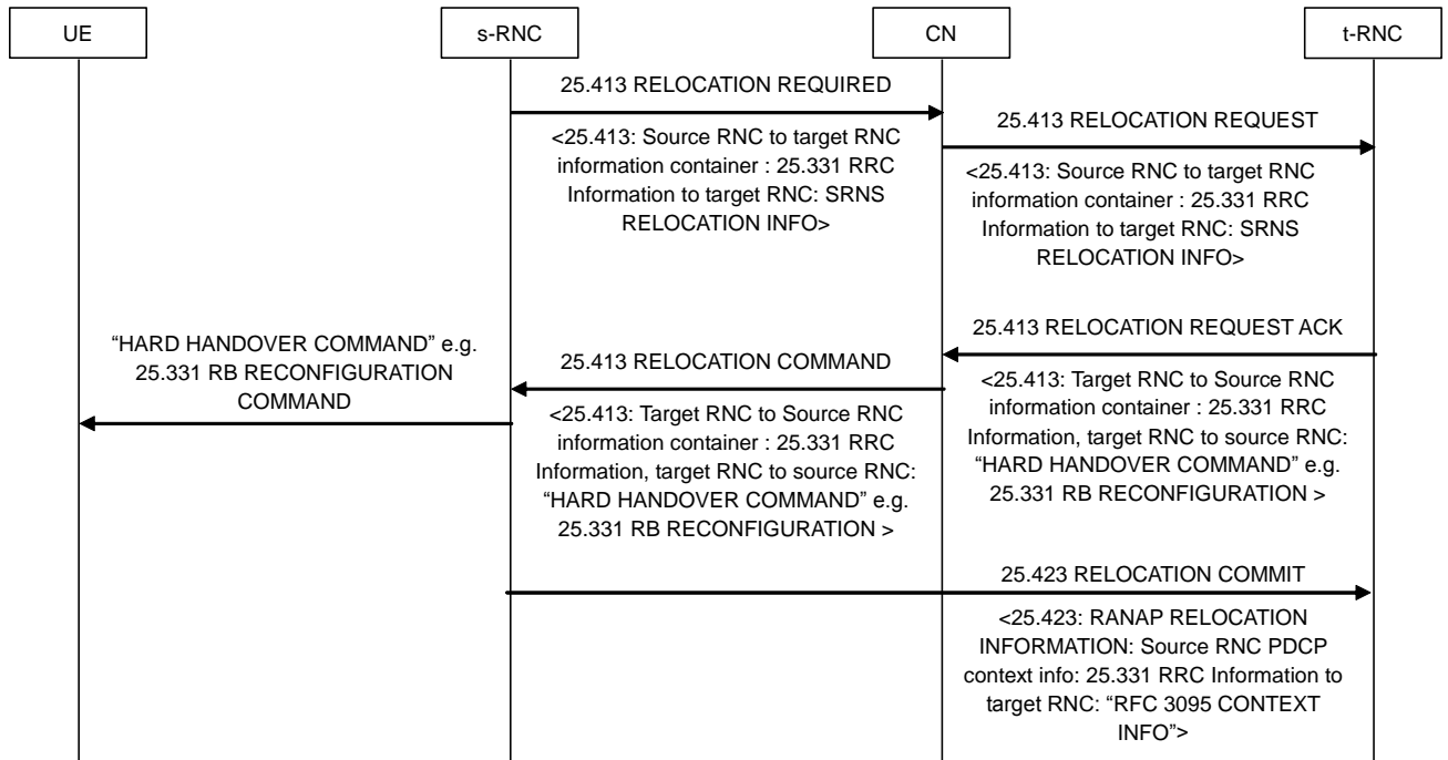
Figure 5.1.7.2-3a: SRNS relocation, flow with context relocation info in RELOCATION COMMIT
