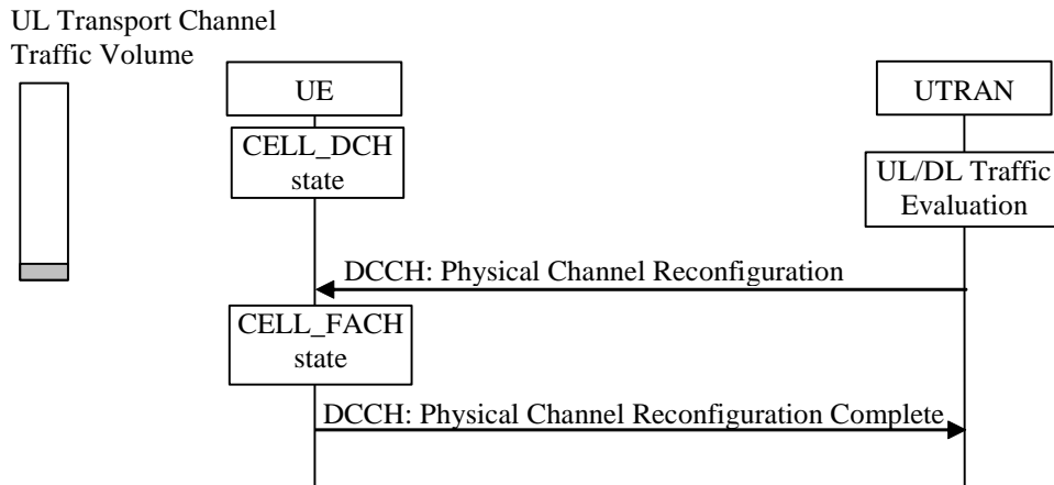
Figure B-5: Physical channel reconfiguration triggered by decreased UL data and with a switch from CELL_DCH to CELL_FACH
