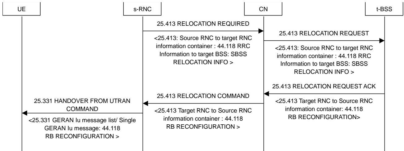
Figure 5.1.7.2-2a: Handover from UTRAN to GERAN lu mode, normal flow
