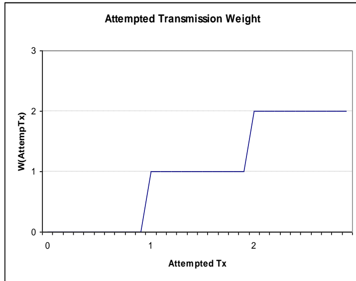
Figure J-4: Attempted transmissions function
