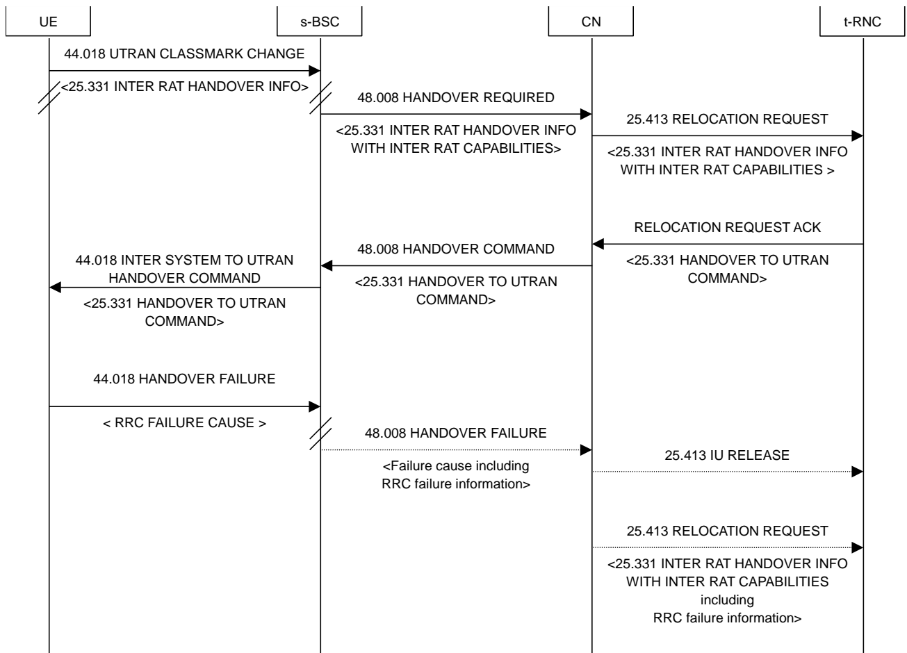
Figure 5.1.7.3-1: Handover of CS domain service from GERAN A/Gb mode to UTRAN, failure due to critical extension not supported by UE
