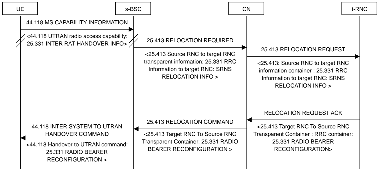
Figure 5.1.7.2-1a: Handover from GERAN lu mode to UTRAN, normal flow
