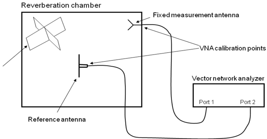
Figure E.2 Calibration measurement setup in the reverberation chamber, using a vector network analyzer.
