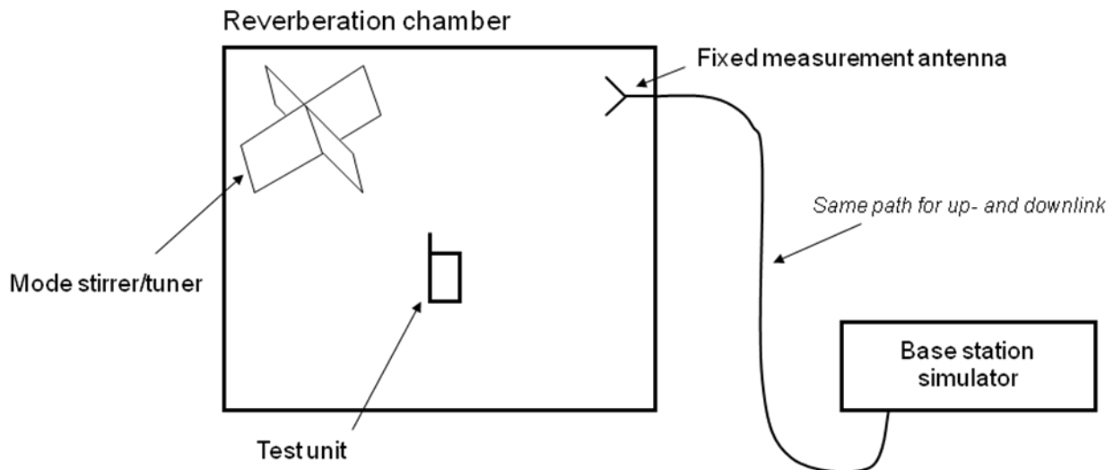
Figure E.1: Schematic picture of the reverberation chamber measurement setup
