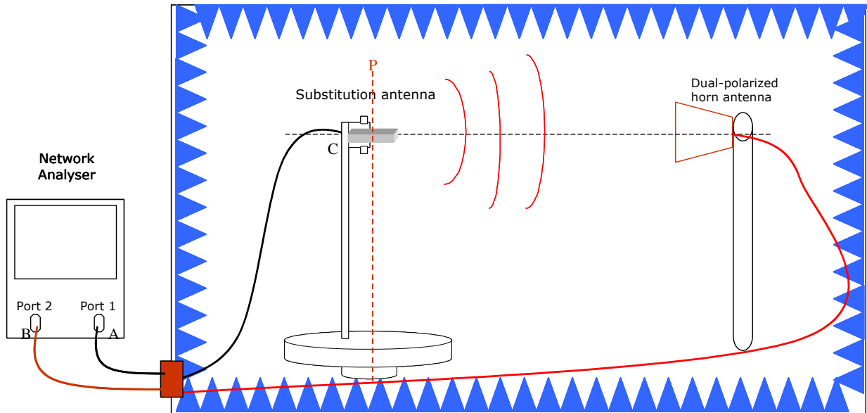
Figure 7.5 Calibration/substitution procedures using a vector network analyzer.
