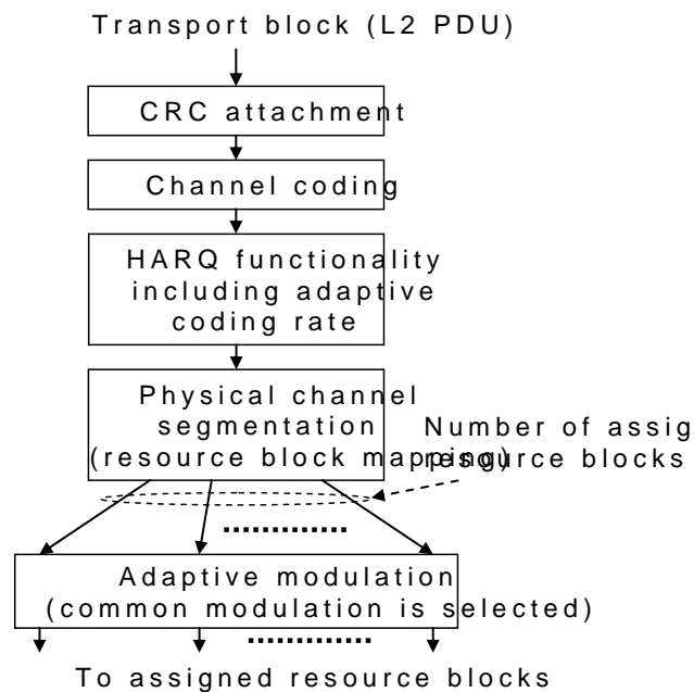
Figure 7.1: Resource block-common adaptive modulation and resource block-common channel coding rate scheme (for localized and distributed transmission modes).
