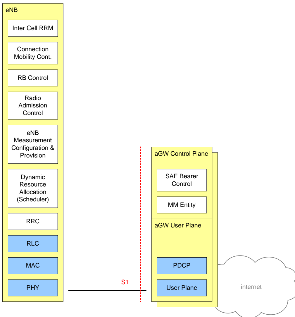
Figure 6.1: E-UTRAN Architecture
