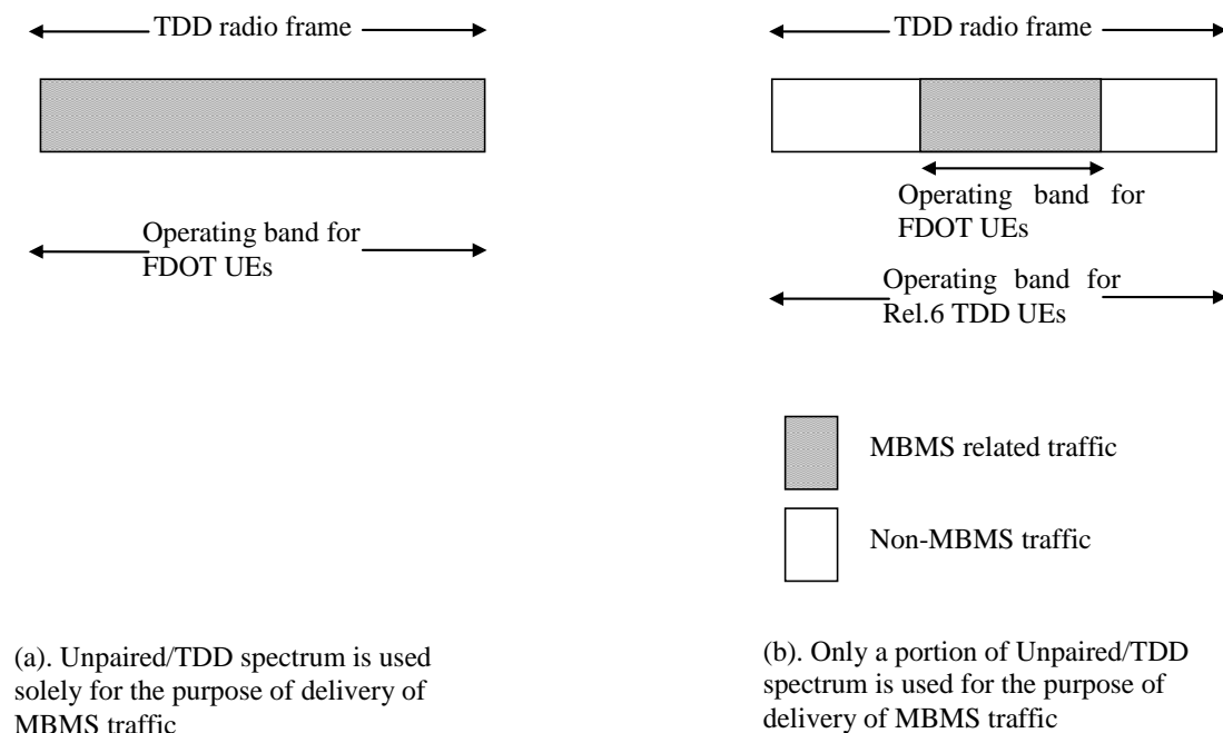
Figure 7: Delivery of MBMS over unpaired/TDD spectrum
