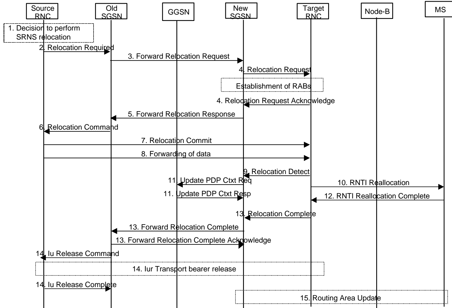
Figure 5: Serving SRNS relocation message sequence (main messages)
