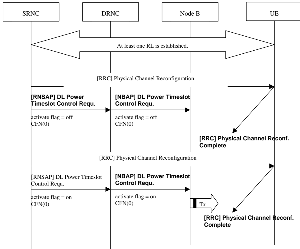
Figure 6: One-shot DL transmit power de-activation/activation(TDD)
