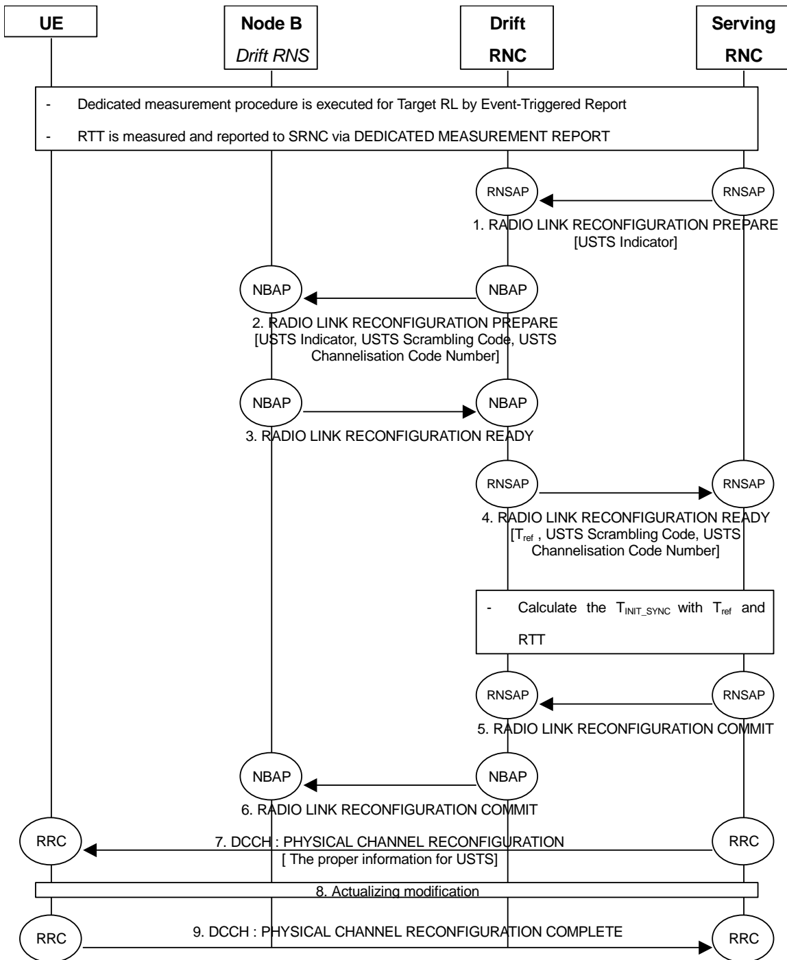
Figure 7. 1 MODE CHANGE procedure
