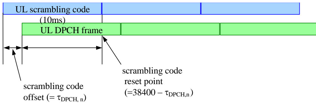
Figure 4.5 Scrambling code offset and reset point (scr. code reference point : P-CCPCH + T_0 + T_{ref} )
