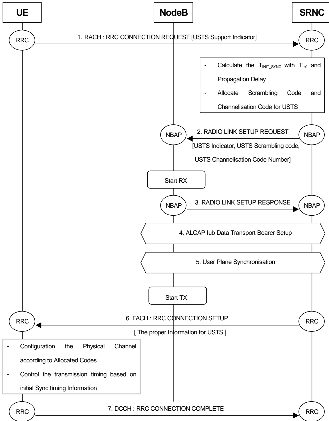
Figure 7. 2 Call Flow of USTS without Iur Interface
