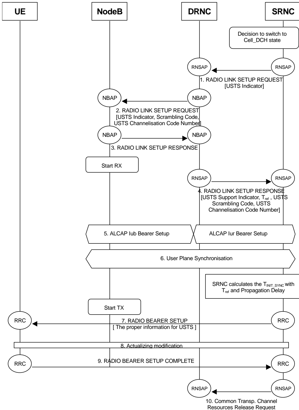
Figure 7. 3 Call flow for State Switching from CELL_FACH to CELL_DCH
