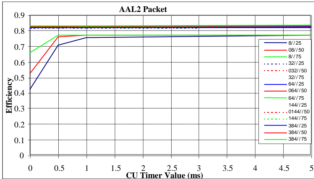
Figure 5: AAL2 Transmission Efficiency 2
