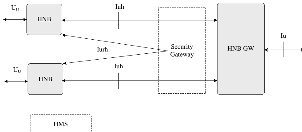
Figure B.1-2. HNB access network deploying Iurh connectivity via a Security Gateway.
