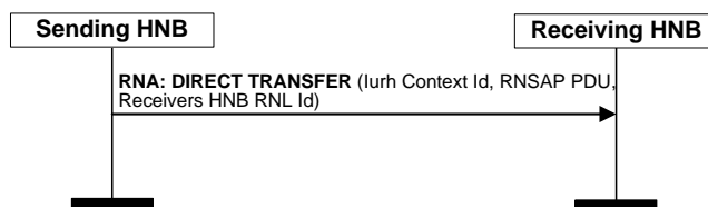
Figure 7.3.2.3.1-1: Transport of RNSAP messages via an established lurch signalling connection – Direct lurch connectivity.
