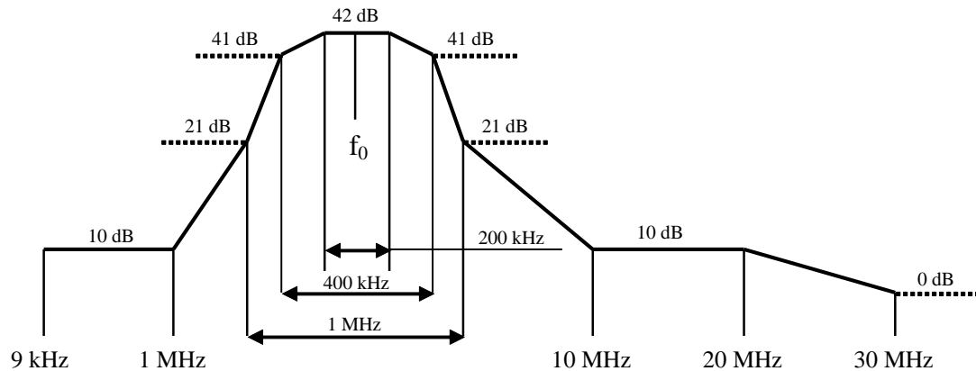
Figure 4.3.1.2.1: Modem attenuation
