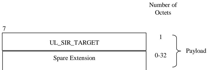
Figure 34: Structure of the payload for OUTER LOOP PC control frame
