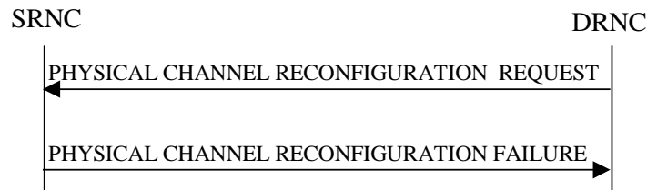
Figure 17: Physical Channel Reconfiguration procedure, Unsuccessful Operation
