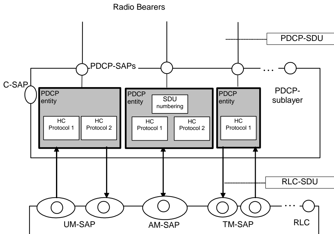
Figure 1: PDCP structure
