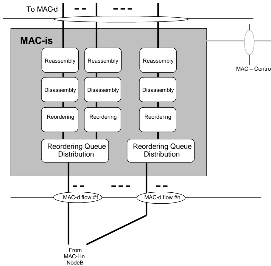
Figure 4.2.4.7-2: UTRAN side MAC architecture / MAC-is details (TDD)
