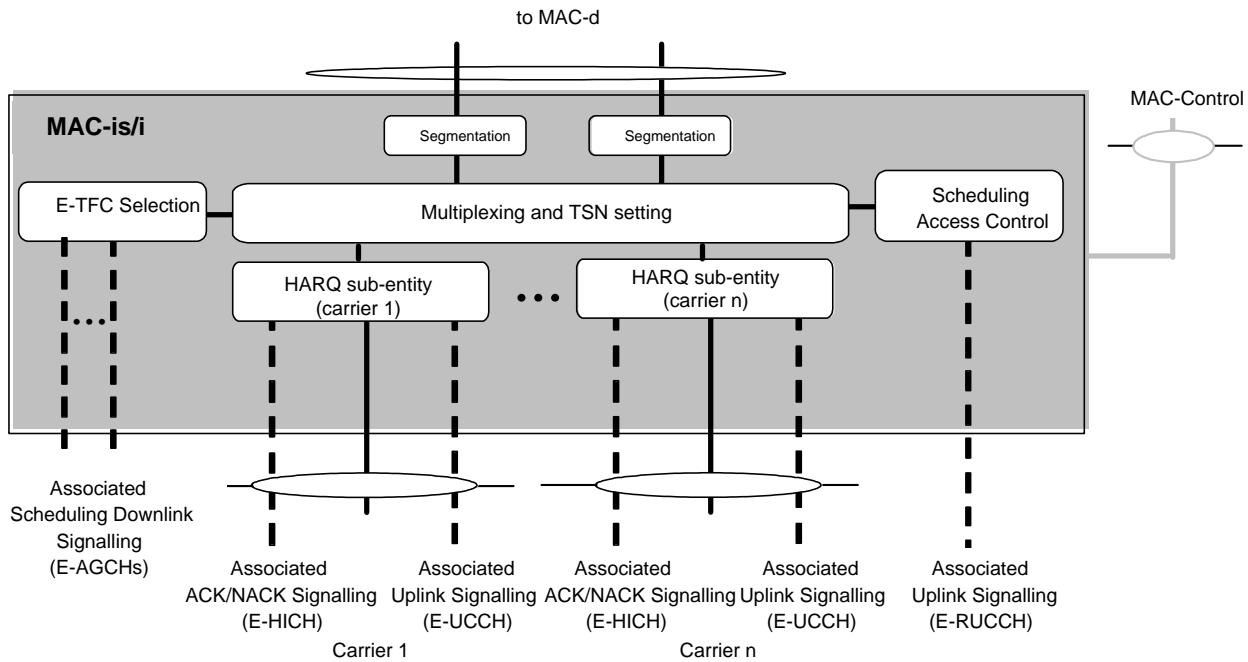
Figure 4.2.3.6-2a : UE side MAC architecture/MAC-i/i details (1.28Mcps TDD multi-carrier E-DCH carrier is configured)
