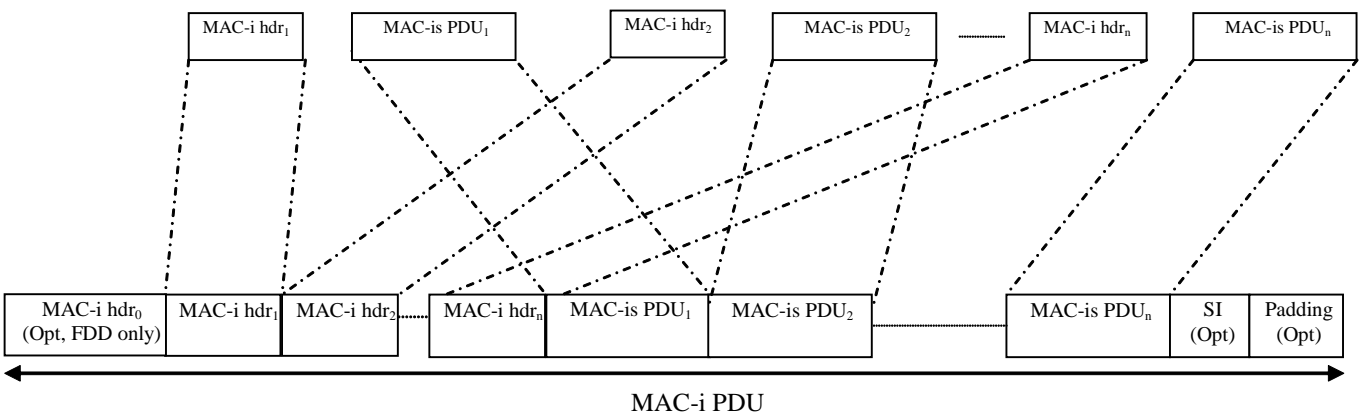
Figure 9.1.5.3 MAC-is PDU.
