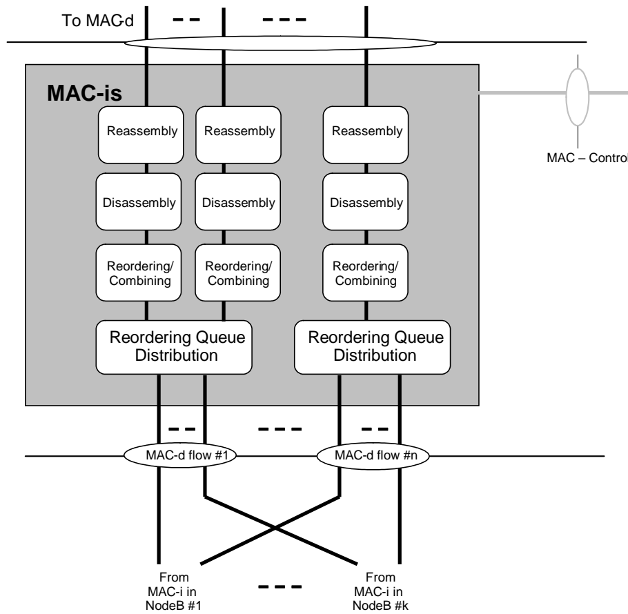
Figure 4.2.4.7-1: UTRAN side MAC architecture / MAC-i details for DCCH/DTCH transmission (SHO case, FDD only)
