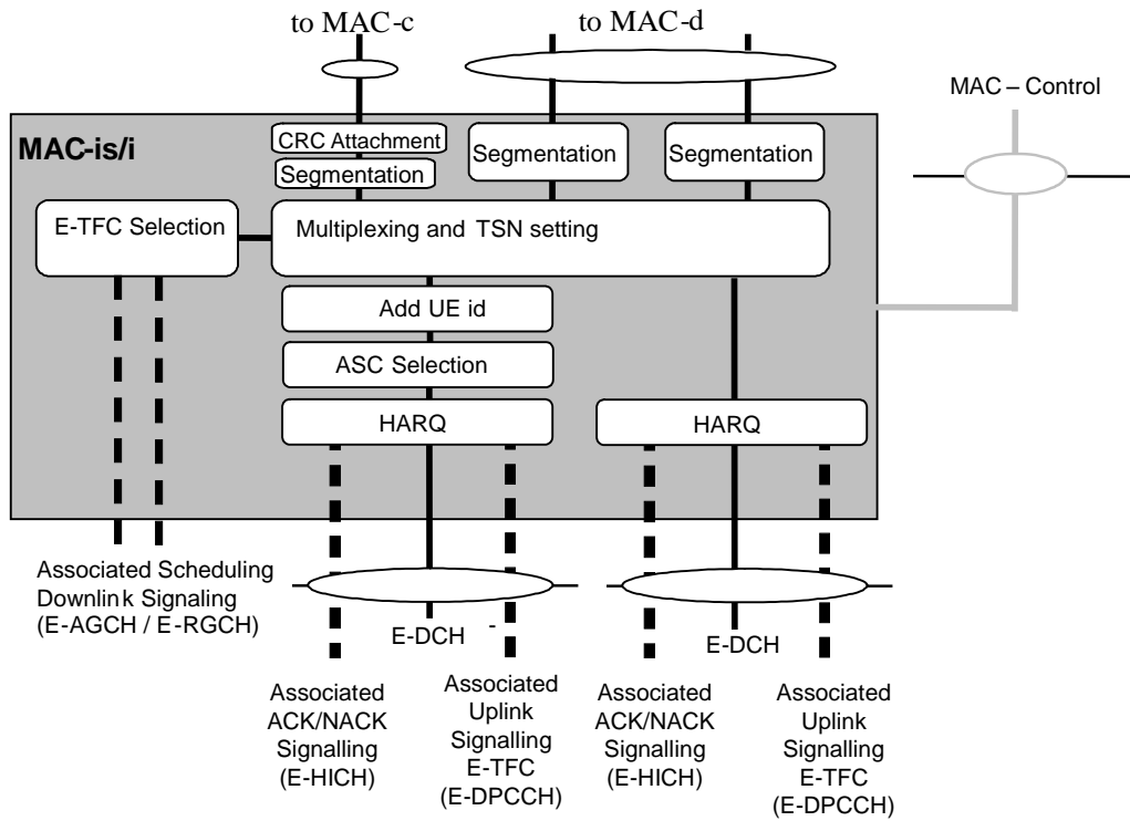
Figure 4.2.3.6-1: UE side MAC architecture / MAC-i/i details (FDD)
