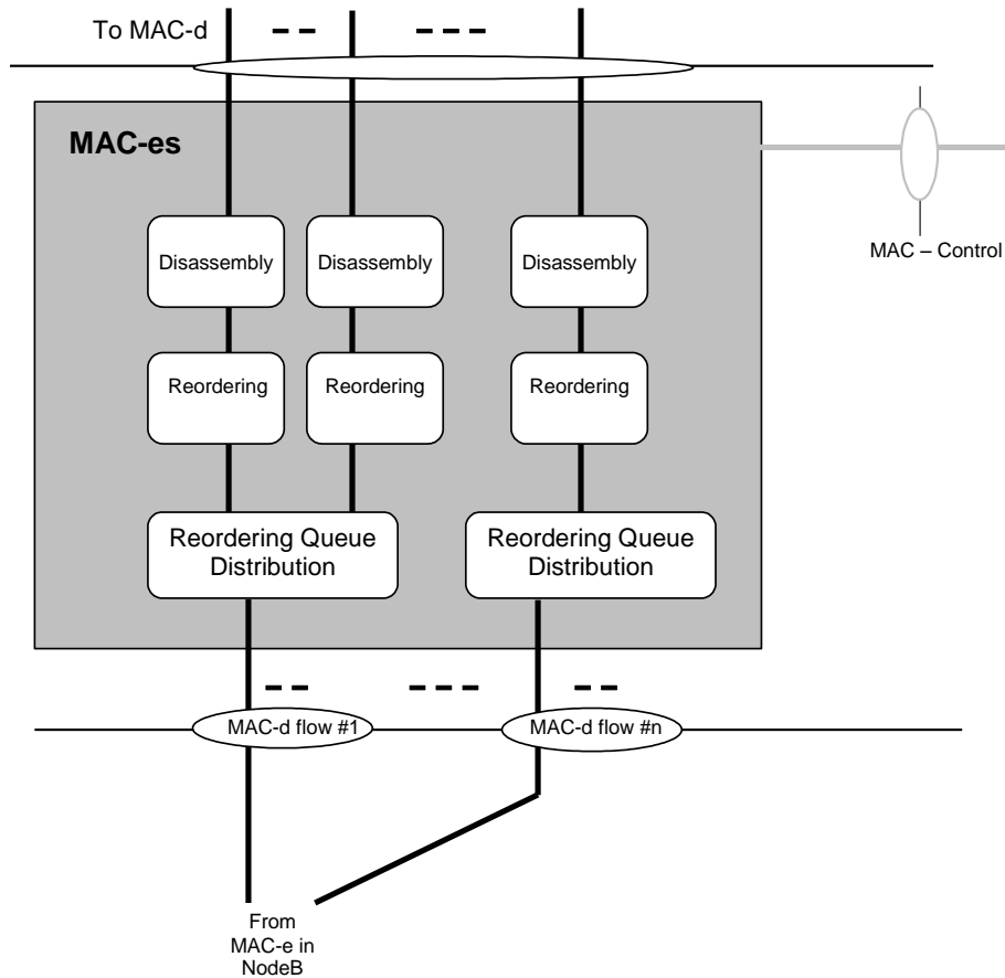
Figure 7.3.5-2: UTRAN side MAC architecture / MAC-es details (TDD only)
