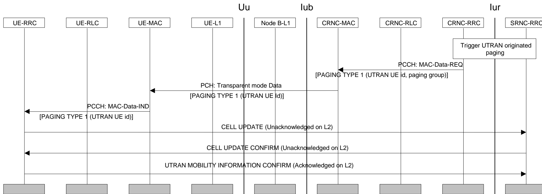
Figure 42: Example sequence for UTRAN initiated paging request with paging response
