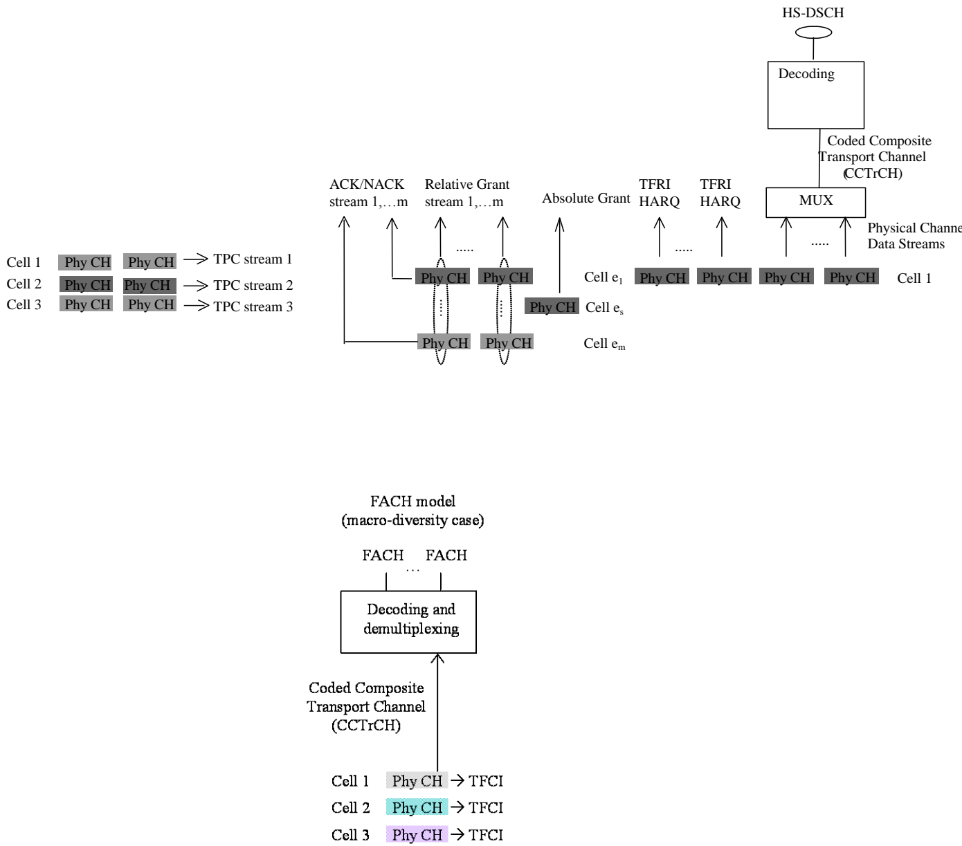
Figure 3: Model of the UE's physical layer - downlink FDD mode
