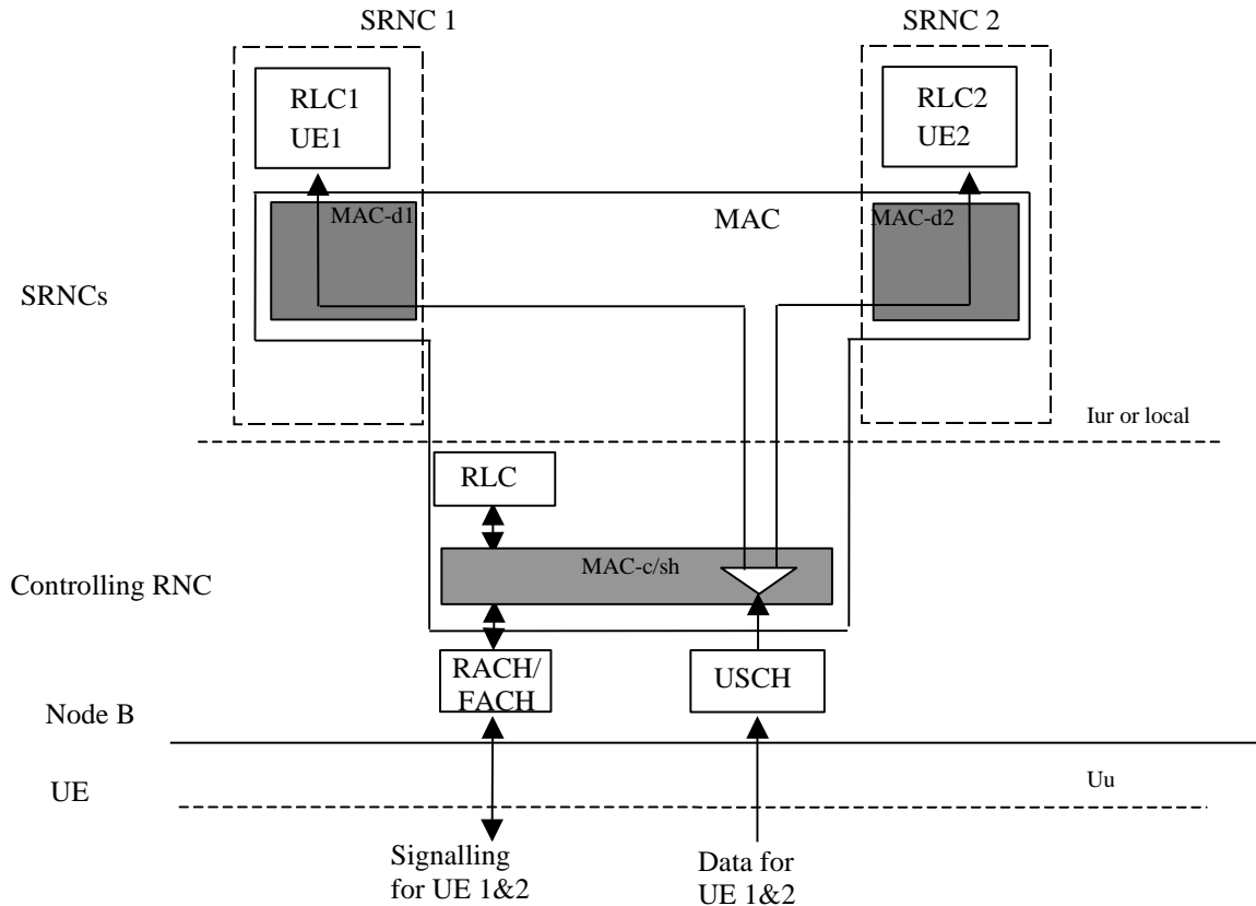
Figure 18: Model of uplink shared channel (USCH) in UTRAN (TDD only)
