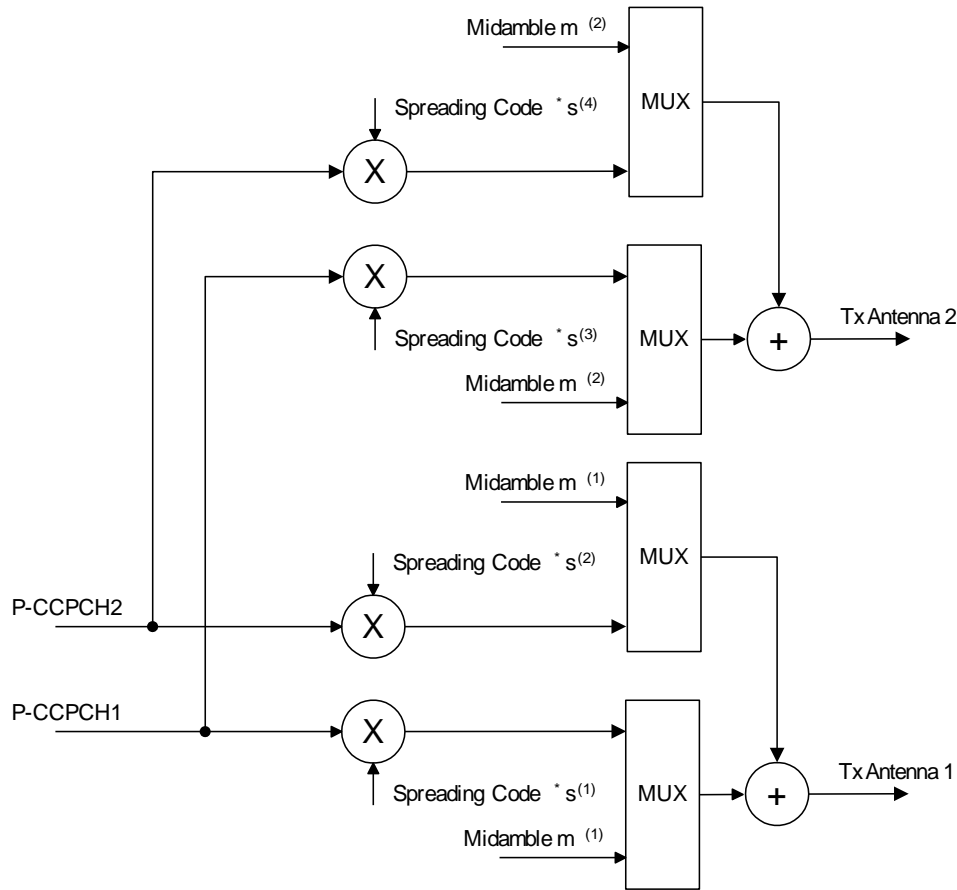
Figure 10: Block Diagram of the transmitter (SCTD) in 1.28 Mcps TDD, exemplary for the P-CCPCH
