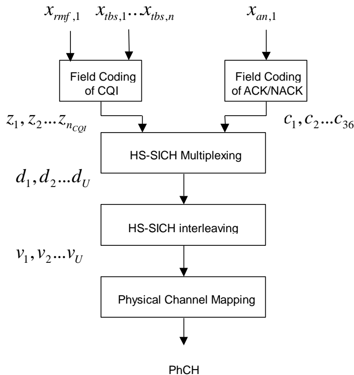
Figure 20: Coding and multiplexing for HS-SICH
