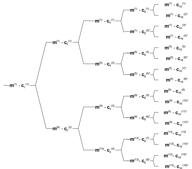
Figure AA.3.1aa: Association of Midambles to Spreading Codes for K=16 pattern 1A
