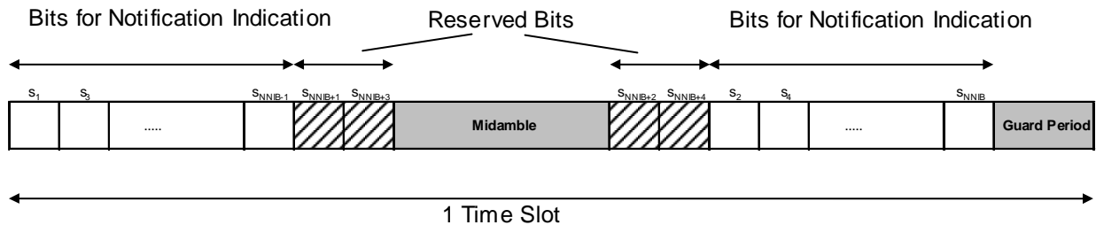
Figure 17a: Transmission and numbering of MBMS notification indicator carrying bits in a MICH burst using burst types 1 and 2
