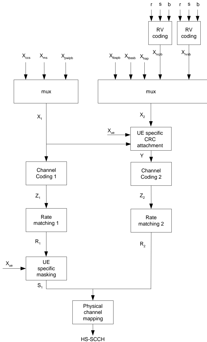
Figure 19B: Coding chain for HS-SCCH type 3
